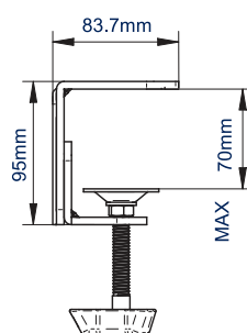
DESK CLAMP
